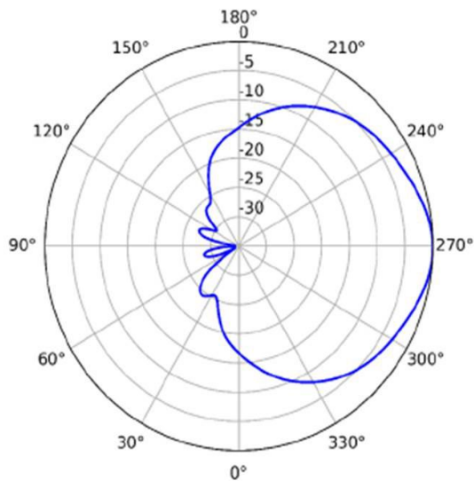
2.4GHz (Horizontal)
